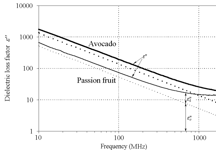
Figure 5. Measured \epsilon'' (solid) and calculated \epsilon_{\sigma}'' (dotted) of avocado and passion fruit as a function of frequency at 20°C. The difference between \epsilon'' and \epsilon_{\sigma}'' represents the contribution from the dipole rotation of polar molecules ( \epsilon_d'' ).
