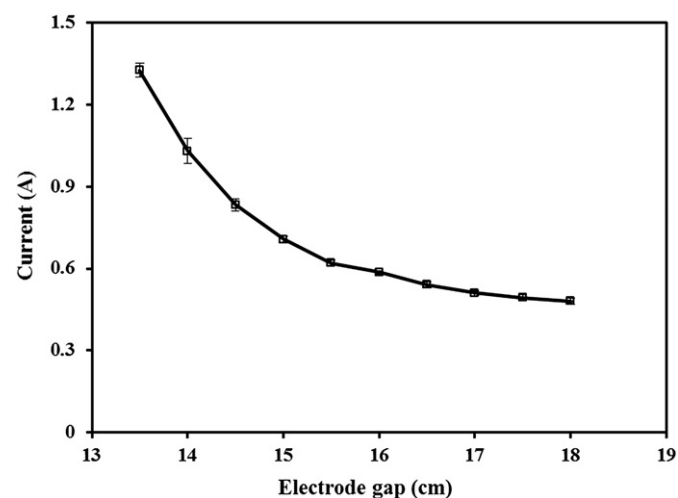
Fig. 4. The relationship between the electrical current and electrode gap with three containers filled with lentils without movement and forced hot air.
