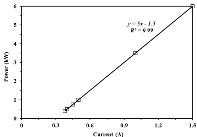
Fig. 3. The relationship between the output power and electrical current of the 6 kW RF unit obtained by Strayfield International, UK using water loads.
