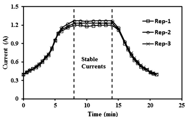
Fig. 7. The electric current change profile when 8 containers passed through the RF unit electrodes with the gap of 14.0 cm.
