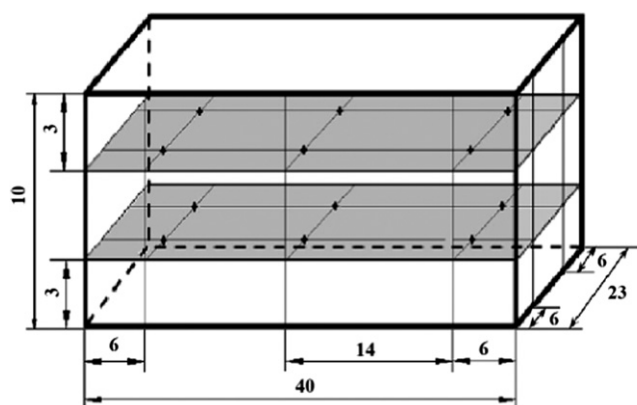
Fig. 2. Dimensions of the plastic container and the location of 12 thermocouples (+) used for temperature measurement (all dimensions are in cm).
