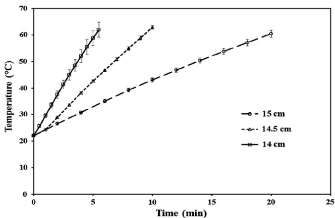
Fig. 5. Temperature-time histories of the RF heated lentils in the geometric center of the middle container under three different electrode gaps without movement and forced hot air.
